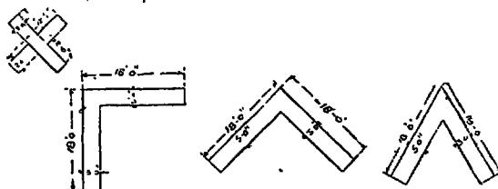
FIG. 1.—DETAILS OF CORNER BRACKETS.
